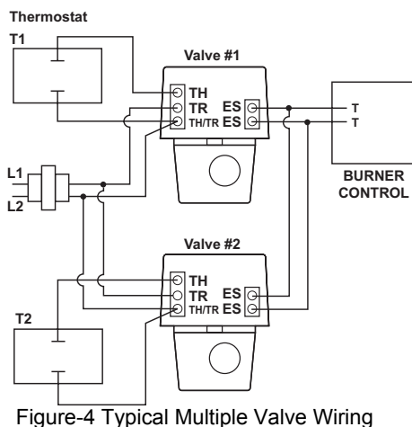
Figure-4 Typical Multiple Valve Wiring
