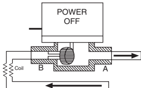
Figure-6a 2-Way Valve With Normally Closed Actuator
