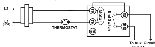
Figure-3 Typical Wiring of a PopTop to Replace a Flair or Taco 3-Wire Valve
